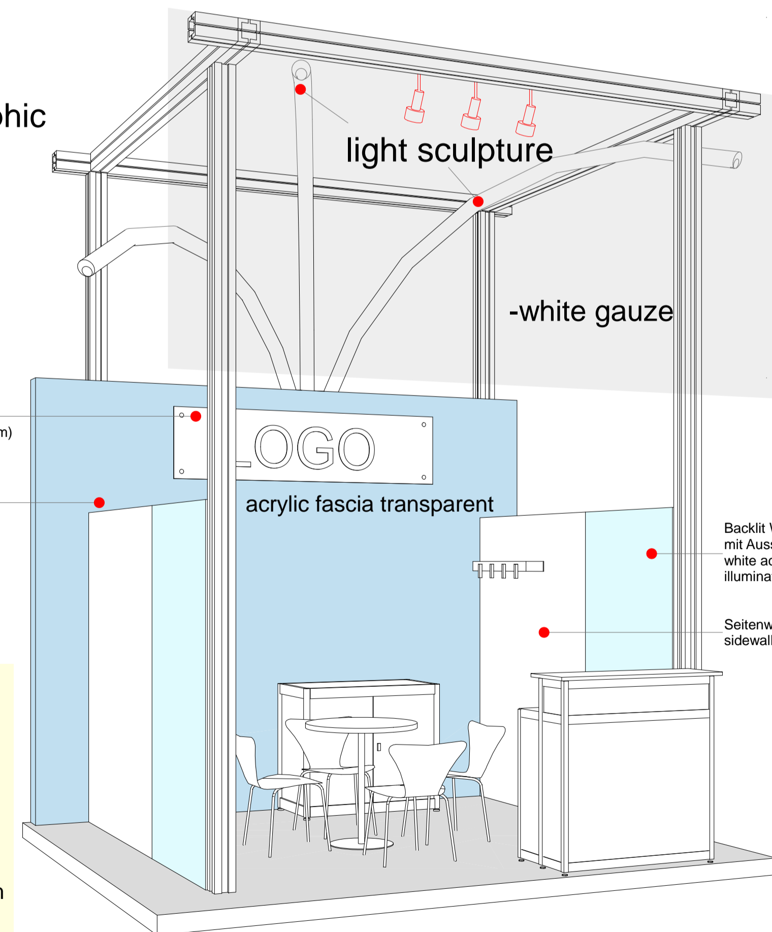
Perspektive/ perspective
