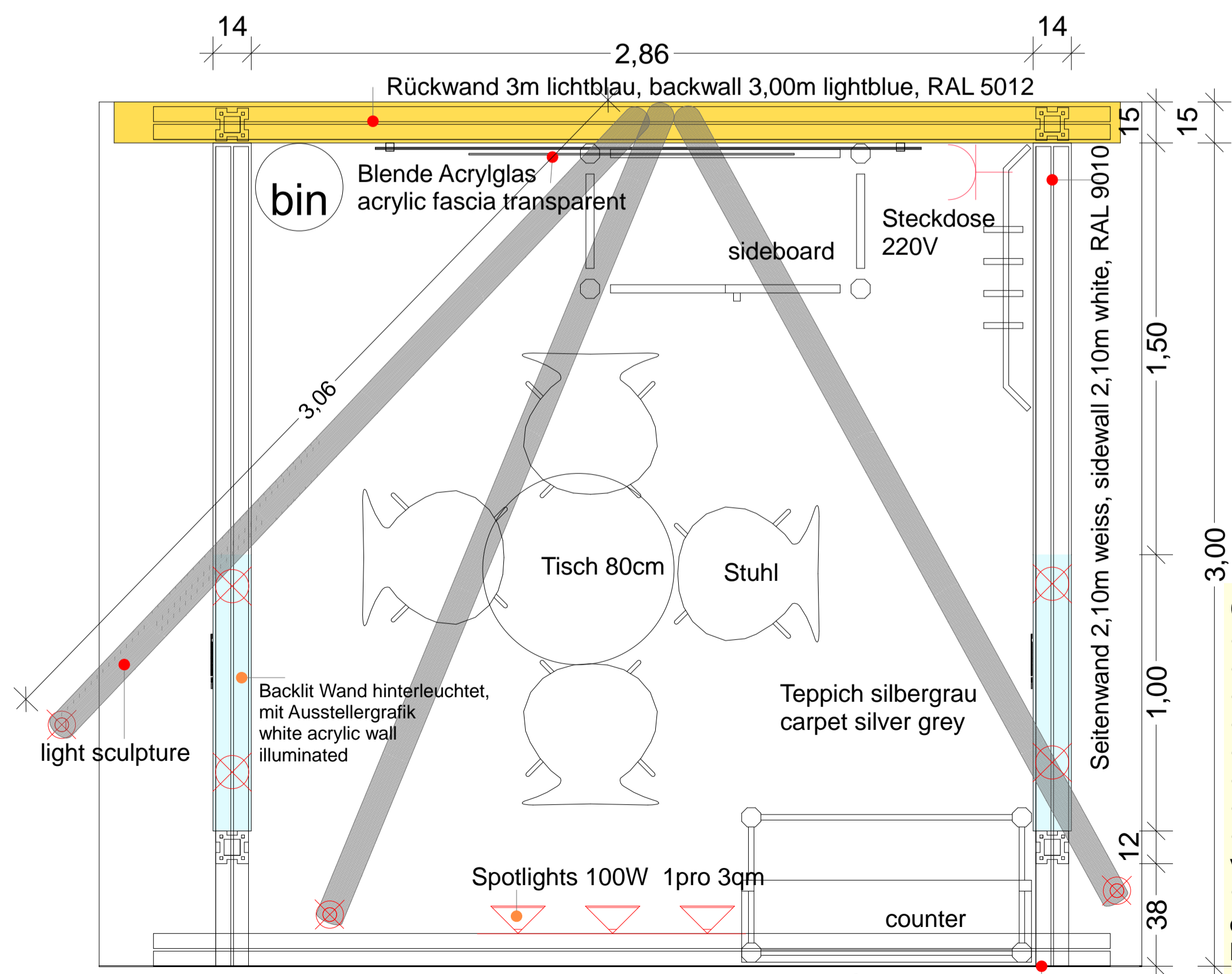
Grundriss/top view
