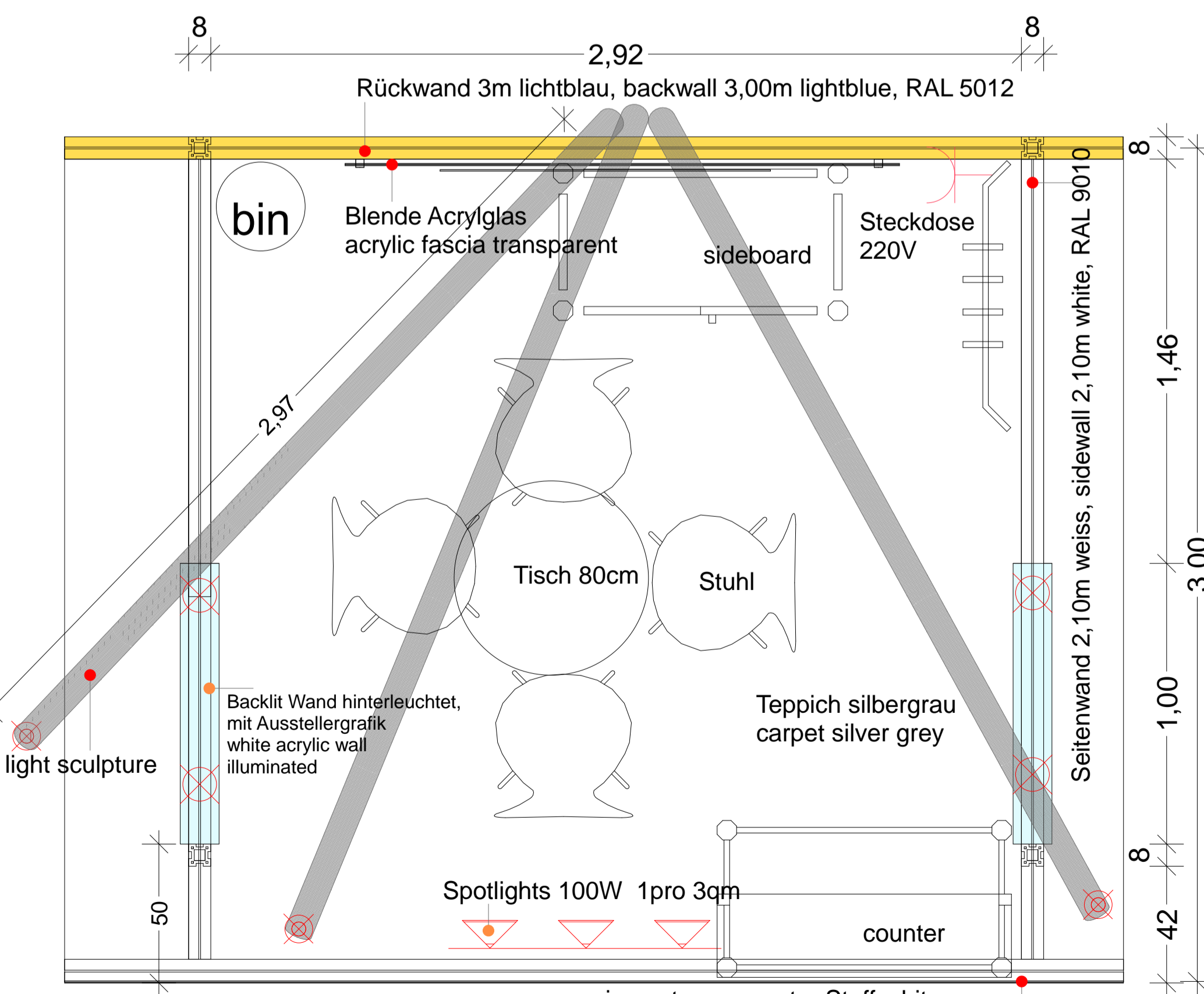
Grundriss/top view Firmenstand Schema - Company booth - 9qm
