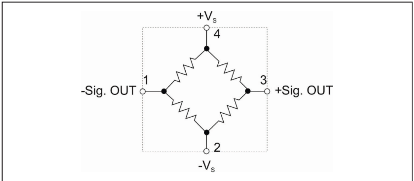
Figure 1: Equivalent circuit
